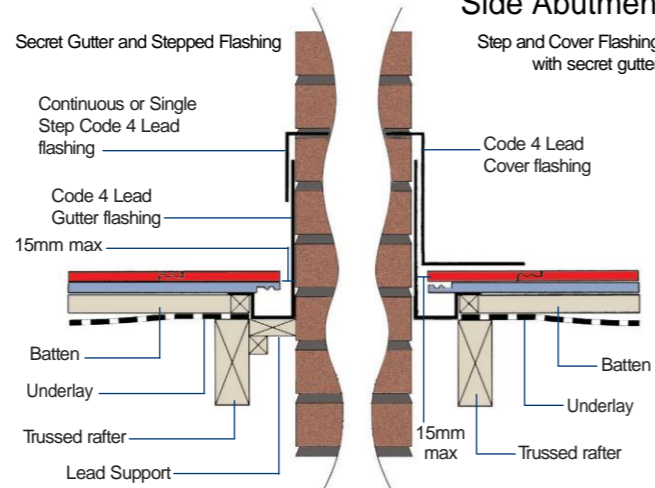
Side Abutment
